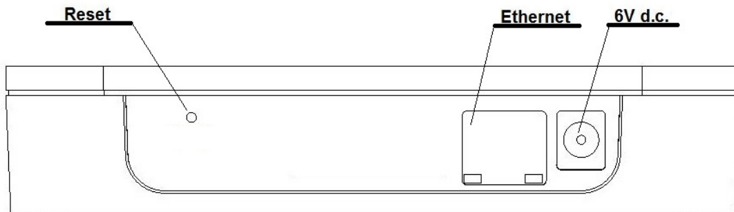
Fig. 3. View of the upper part of HT20IoT monitor
