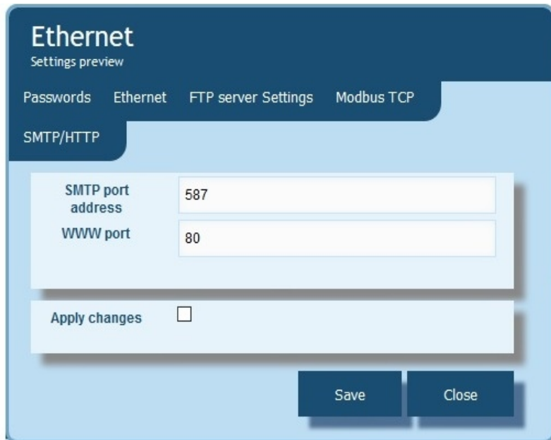
Fig. 18. View of FTP ports configuration window
