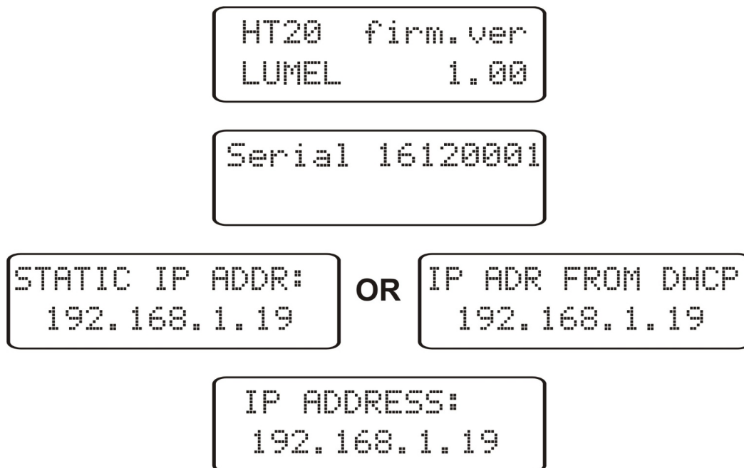
Fig. 4. Startup messages of HT20IoT monitor
